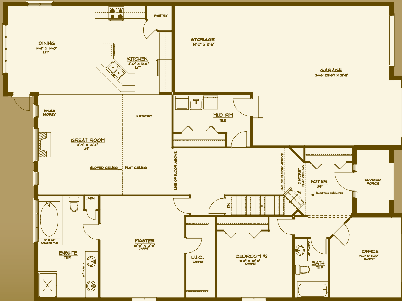
Main Floor • 2,189 Sq. Ft.
