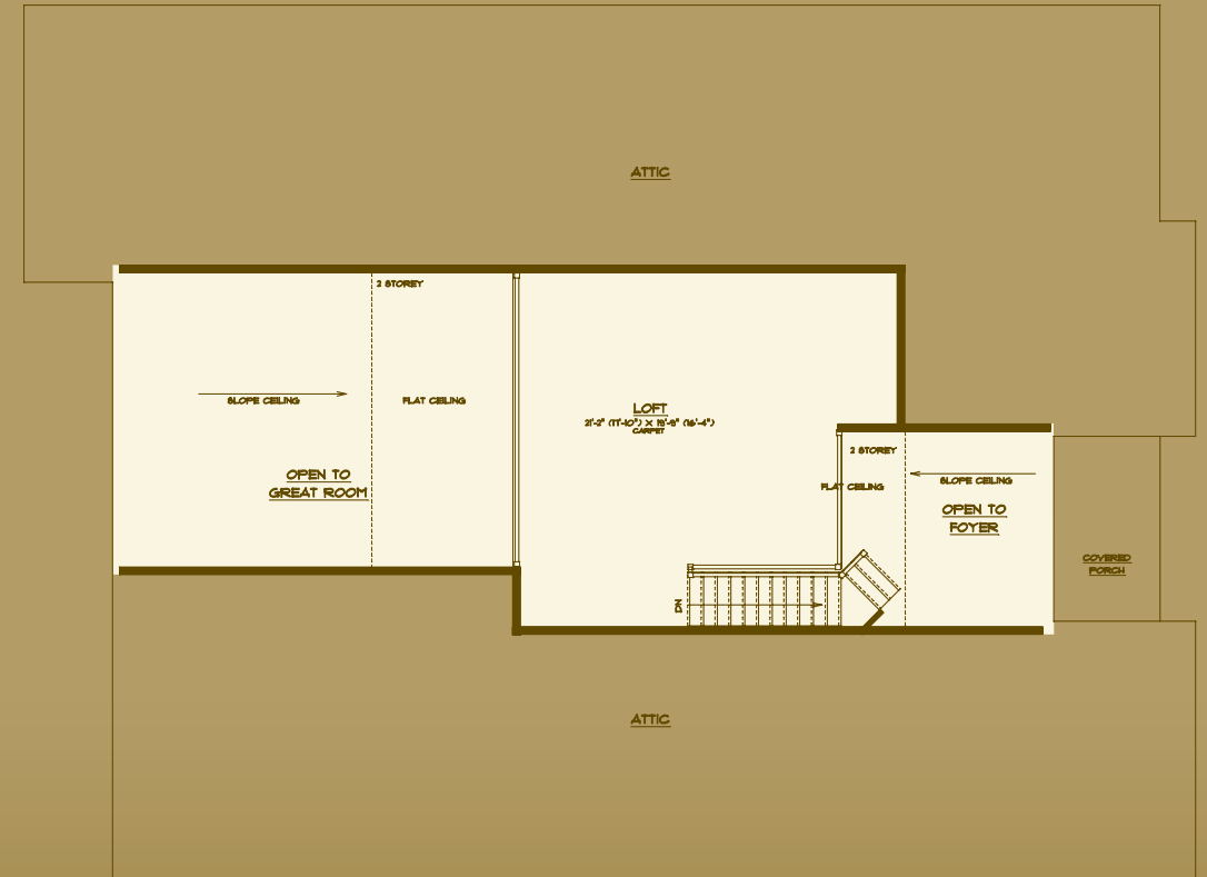
Loft Floor • 592 Sq. Ft.
